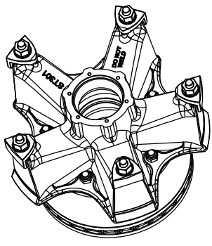
AUXILIARY VIEW OF HUB ASSEMBLY
