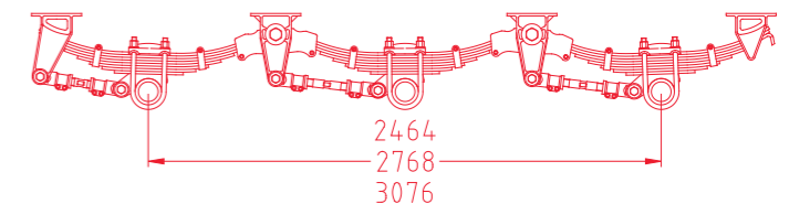
TRI-AXLE
