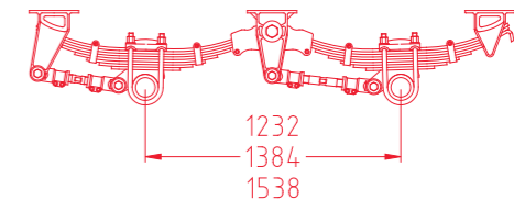
TANDEM AXLE
