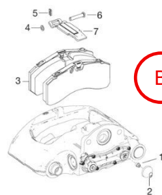
PAD SET (1 AXLE): Knorr-Bremse
