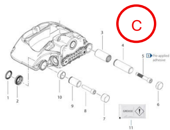
SEAL KIT (1 CALIPER): Knorr-Bremse
