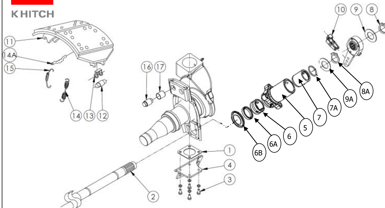
BRAKE AND KNUCKLE COMPONENTS DRUM BRAKE
