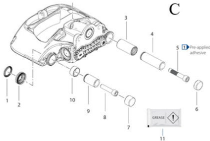
SEAL KIT (1 CALIPER): Knorr-Bremse
